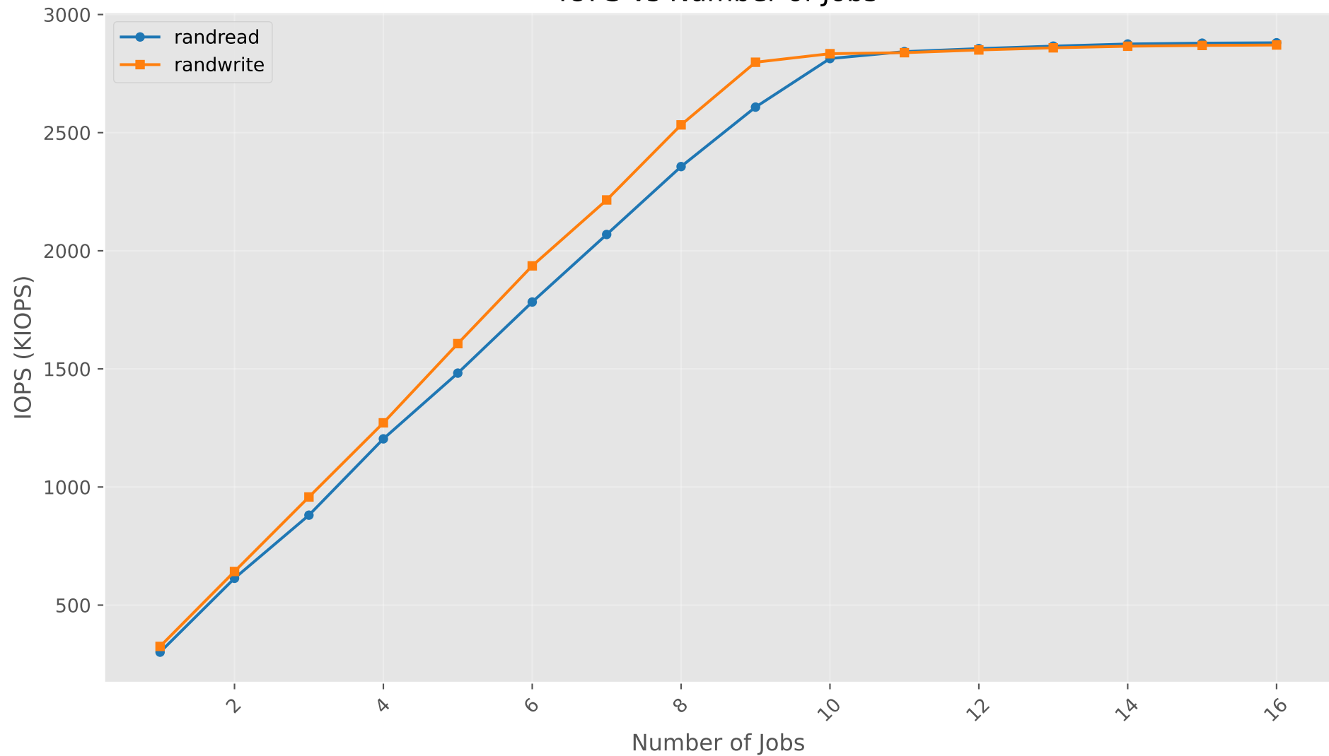
IOPS vs Number of Jobs
